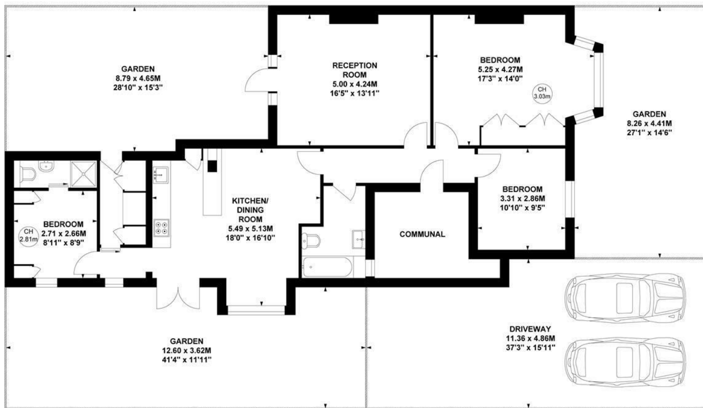
Ground Floor
